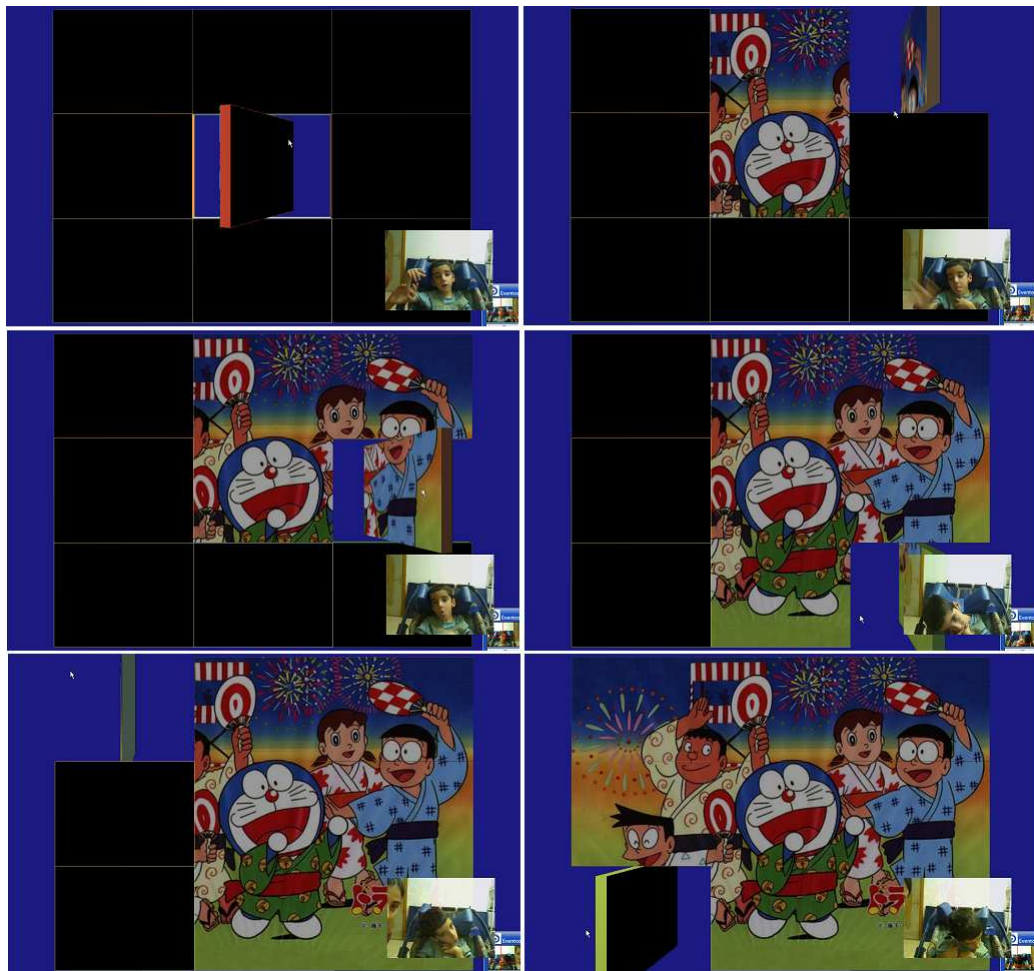
Figure 4.6: Test 3.
