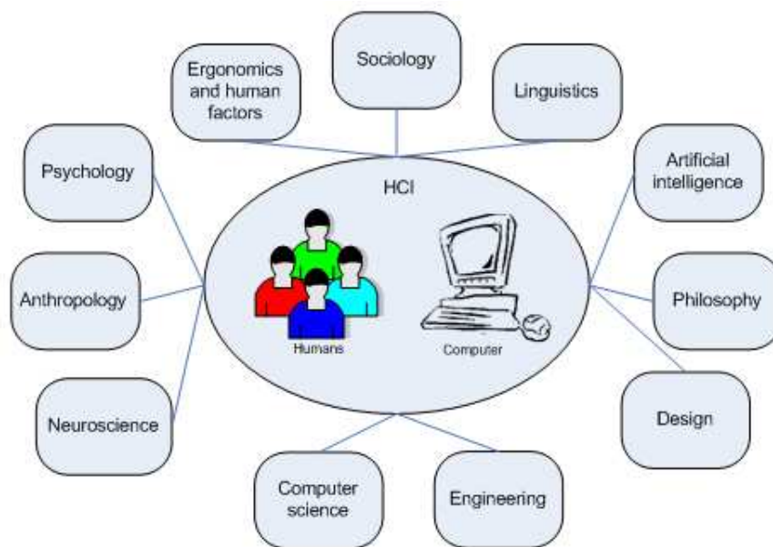
Figure 2.2: HCI fields.
