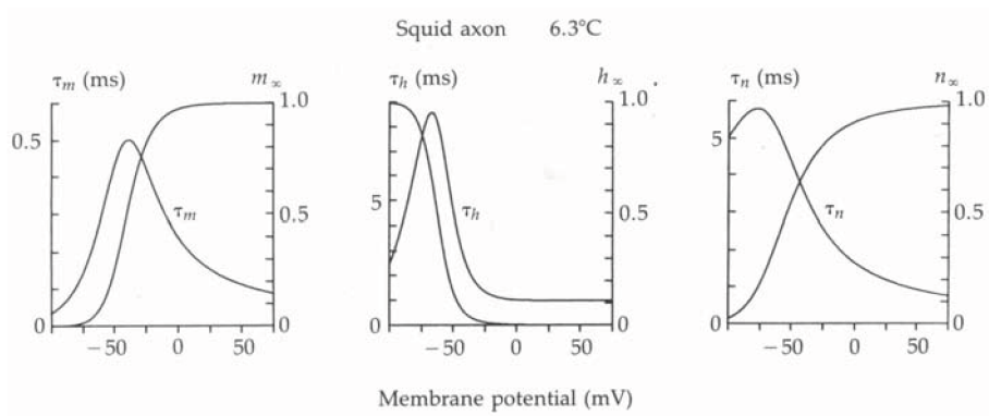
Figure 1.12: Voltage-dependent time constants \tau_m , \tau_h and \tau_n and steady-state values m_\infty , h_\infty and n_\infty .
