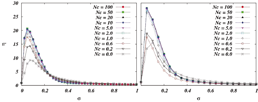
Figure 4.5: Spectral amplification factor \eta as a function of \sigma for an increasing N_c . The ratio of excitatory to inhibitory connections was fixed to 4. Other parameters: a = 0.06 , K = 1.5 and A = 0.05 . (a) T = 1.6 and (b) T = 1.11 .
