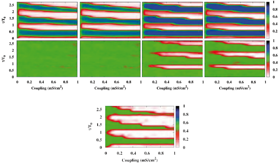
Figure 5.2: Upper panel: Contour plots of S^{loc} (top row) and S^{glob} (bottom row) in the coupling-delay phase space. Columns, from left to right, correspond to simulations with different topologies: regular, small-world, random and scale-free. Bottom panel: Contour plot of S^{glob} for the globally coupled network.
