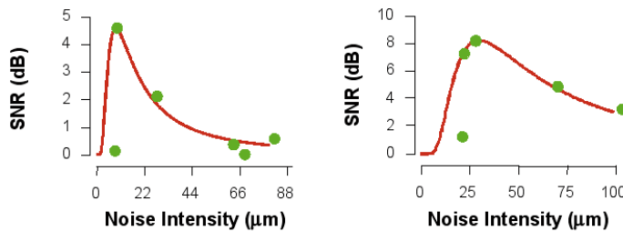
Figure 2.8: Computed signal to noise ratio from experimental data (green dots). Red line stands for the best fit SNR \propto (a/D)^2 e^{b/D} obtained. Both panels correspond to two different realizations of the experiment.
