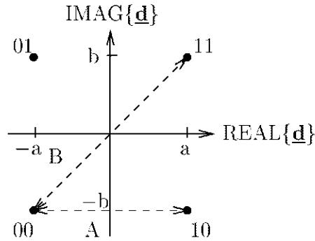
Figure 2.11. 4 PSK modulation.
