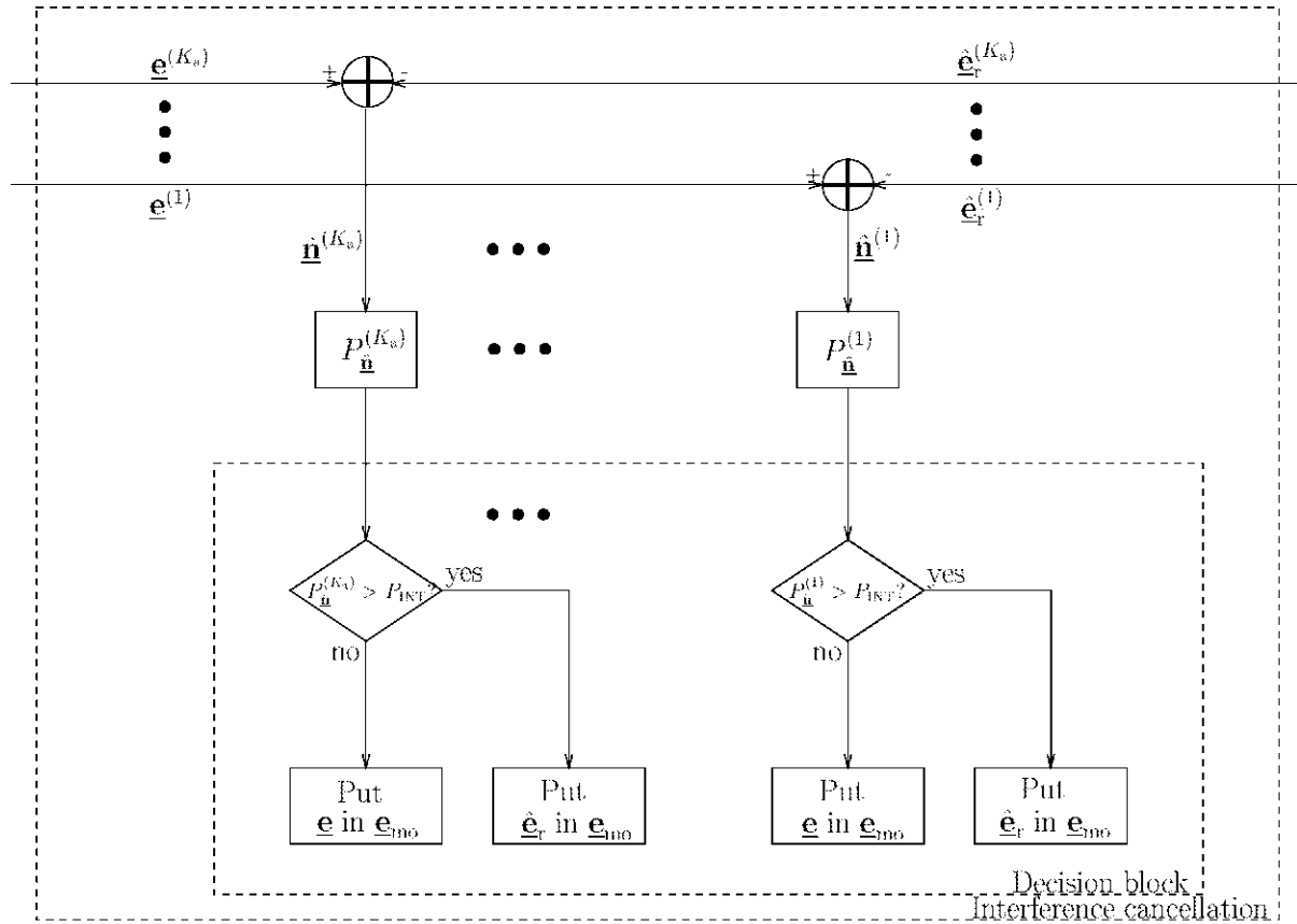
Figure 2.7. Block interference cancellation.
