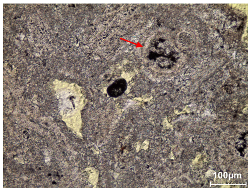
Fig. 15. Preserved foraminiferal test (red arrow) in the incompletely burned limestone fragment (sample E4, X1601).
