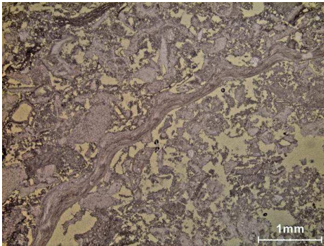
Fig. 6. Photomicrograph of the sample E17 (X1610). Very slightly sandy, coarse porous bioclastic rudstone-floatstone (shell of brachiopod visible in the middle) – Cova de sa Prior, wall of the cave, at the entrance.
