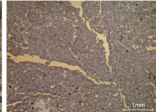
Fig. 11. Photomicrograph of the sample E4 (X1601) – Cova de sa Prior, lime burial (2015).
