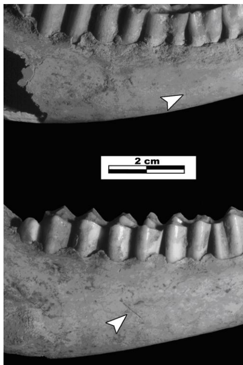
Fig. 7. Caprine humeri with cut marks from Canyamel.
