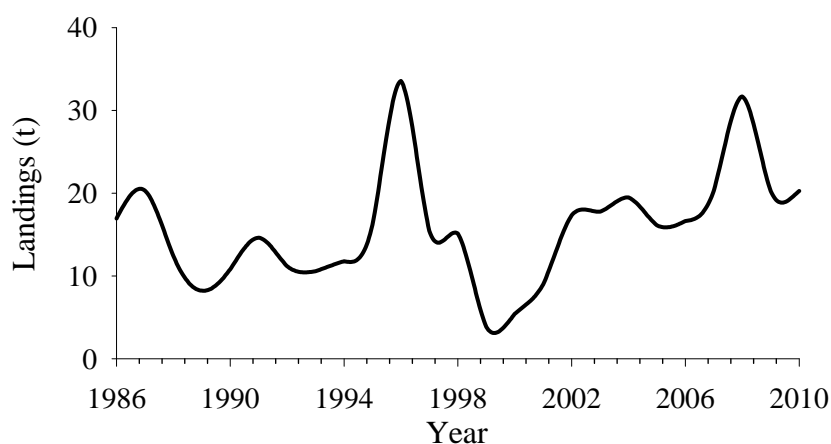
Figure 1.37. Landings of the Norway lobster ( N. norvegicus ) from the bottom trawl fleet from Mallorca (Balearic Islands).
