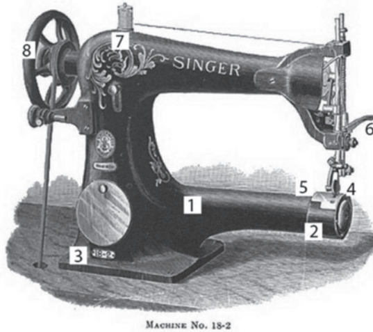
Fig. 4. Màquina de repuntar SINGER 18.2. Instructions for using and adjusting Singer sewing Machines of Class 28. The Singer Manufacturin.
